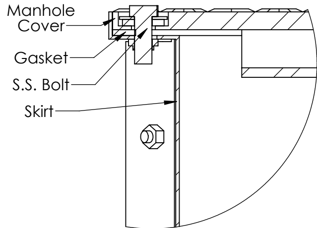
DETAIL R SCALE 1 : 2
